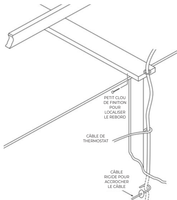
FIGURE 17 - THERMOSTAT
