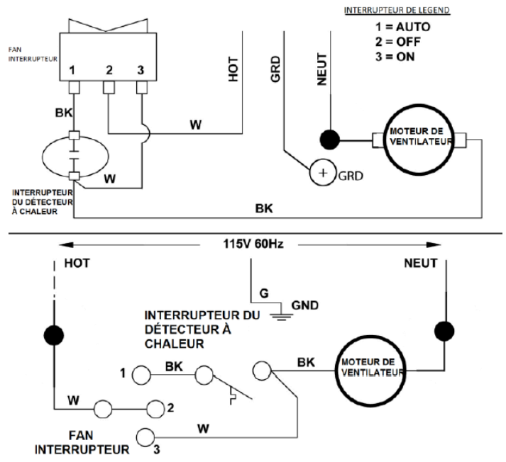
FIGURE 3 - KIT NO. 2303
