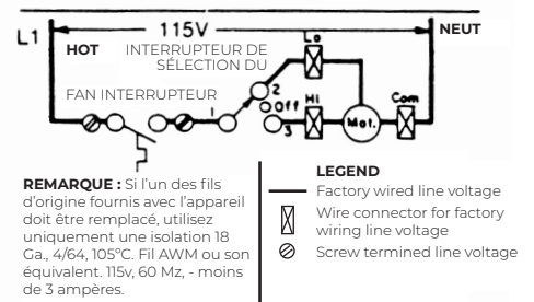
FIGURE 3 - KIT NO. 2303
